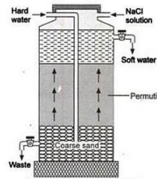
Fig.: Permutit method for softening of hard water
